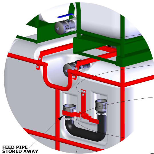
DETAIL C SCALE 1 : 9
