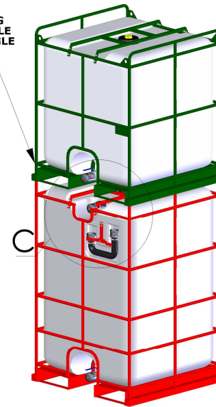
DIMETRIC ILLUSTRATION OF CHEMTAINER AND MOTHER UNIT STACKED
