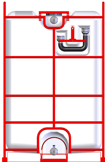
FRONT VIEW OF CHEMTAINER MOTHER UNIT
