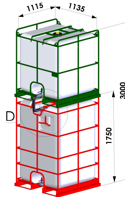
DIMETRIC ILLUSTRATION OF CHEMTAINER AND MOTHER UNIT STACKED AND LINKED
