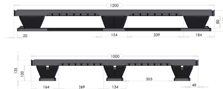
Dimensional Details
